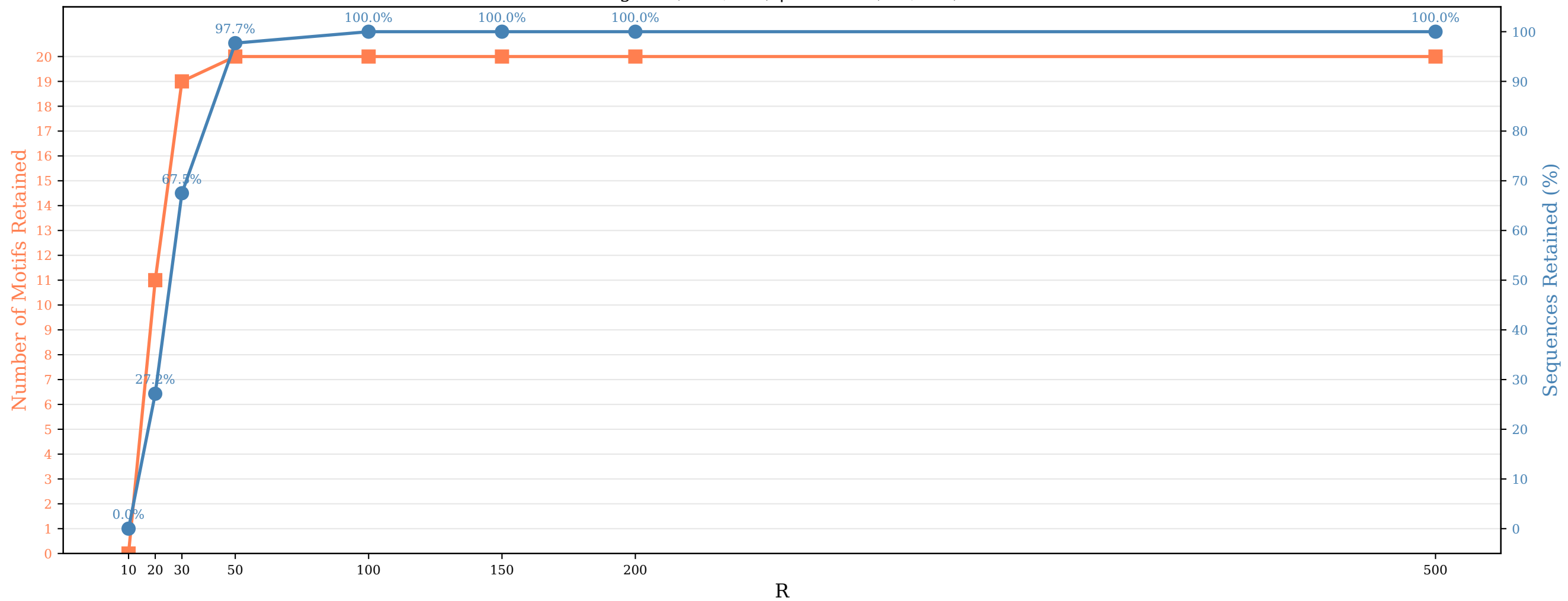
Motif & Sequence Retention vs Neuron Threshold
